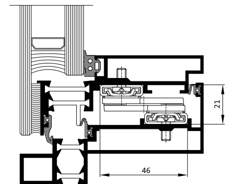
Example of construction: Parallel offset window
